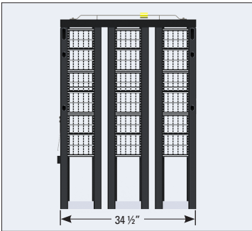
FDP 3434R features a 34 ½” width.
