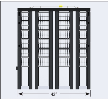
FDP 4334R features a 43” width.
